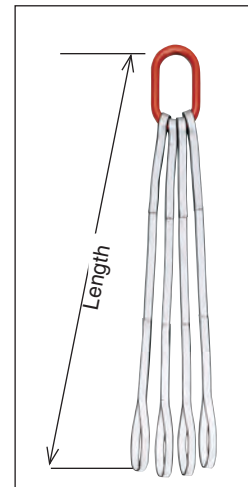
QOE Quad Leg Oblong Link Sling Hook (EE1801T)
