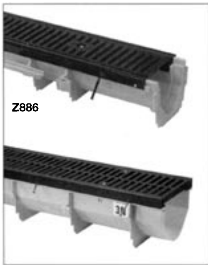
Perma-Trench – 6" and 12" wide pre-sloped polyethylene structural composite systems; catch basins, shallow non-sloped and radiused channel systems.
