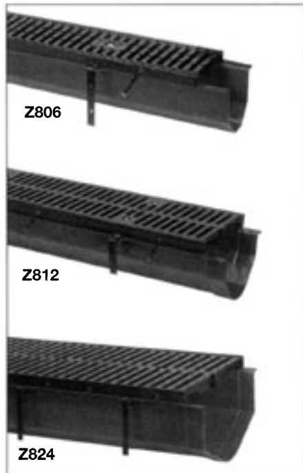
Flo-Thru – 6", 12" and 24" wide pre-sloped fiberglass systems and catch basins.
