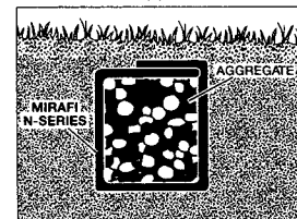
French drain without pipe
